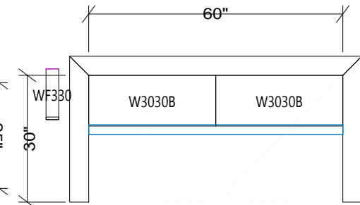
LAUNDRY
