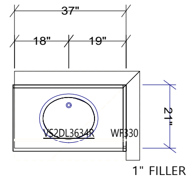
LOWER BATH CABINET HEIGHT 34-1/2"
