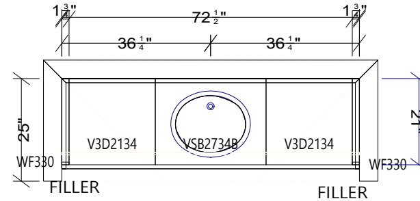
MAIN BATH CABINET HEIGHT 34-1/2"
