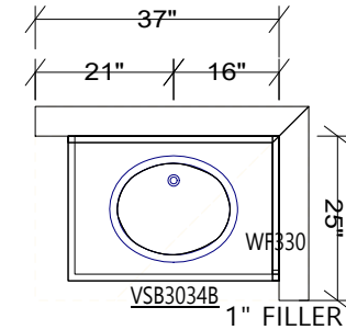
ENTRY BATH CABINET HEIGHT 34-1/2"
