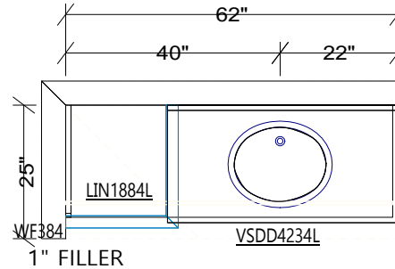
MASTER BATH CABINET HEIGHT 34-1/2"
