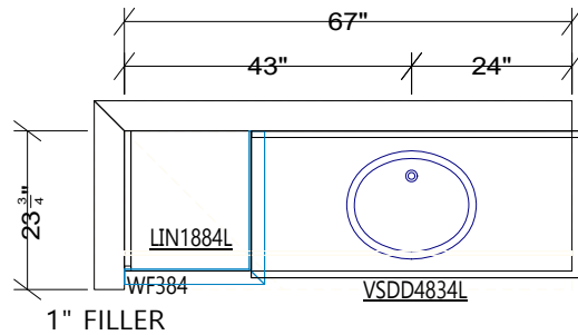
MAIN BATH CABINET HEIGHT 34-1/2"
