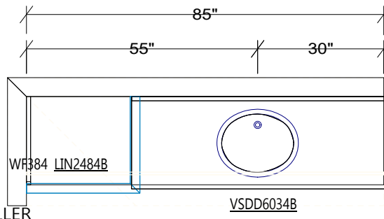
21" DEEP LINEN MASTER BATH CABINET HEIGHT 34-1/2"
