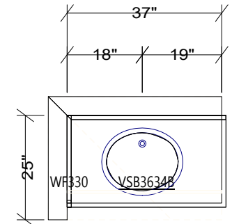
LL BATH CABINET HEIGHT 34-1/2"
