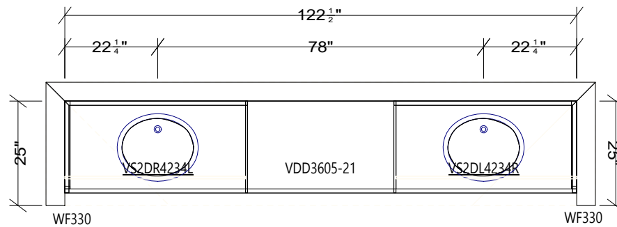
MASTER BATH CABINET HEIGHT 34-1/2" MAKE UP AREA AT 30-1/2"
